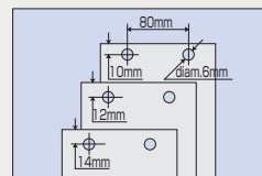
DEPTH GAUGE
